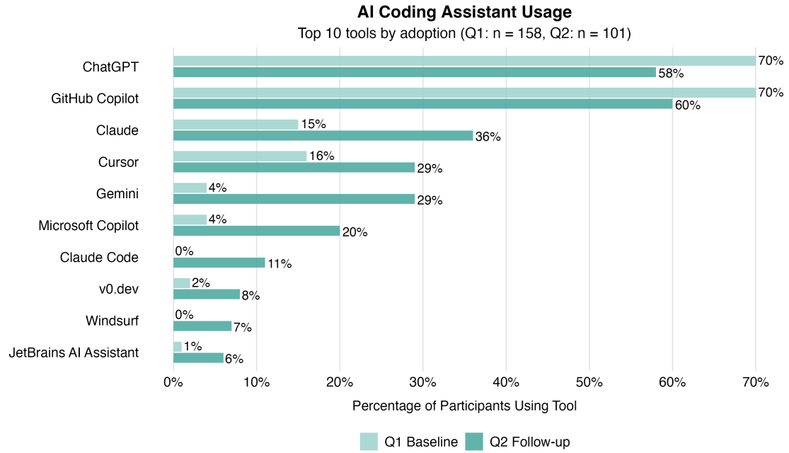
Fig. 1. AI coding assistant adoption rates at Q1 and Q2. Top 10 tools by maximum usage at either time point shown.
