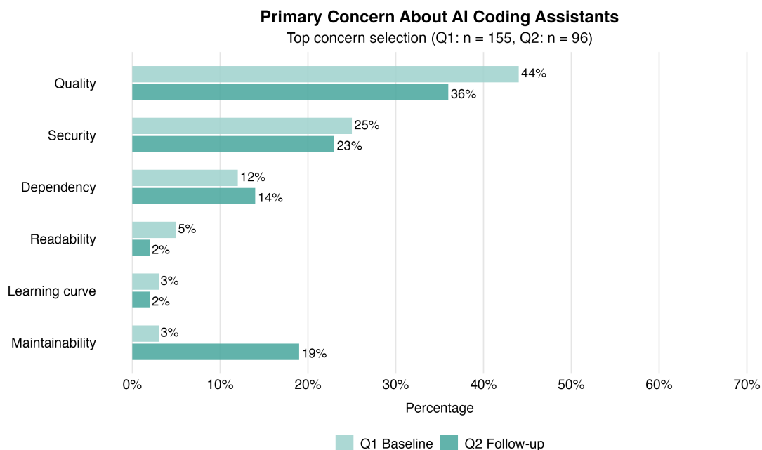
Fig. 4. Primary concern distribution at Q1 and Q2. “Other” excluded from analysis.
