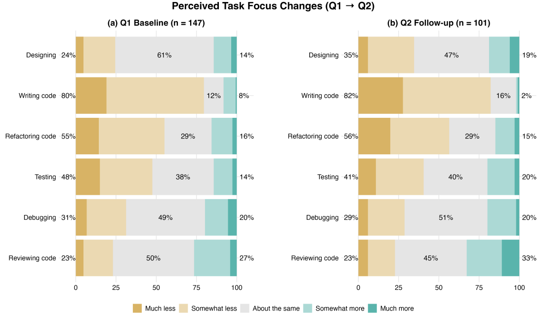
Fig. 5. Task focus shifts across time points.
